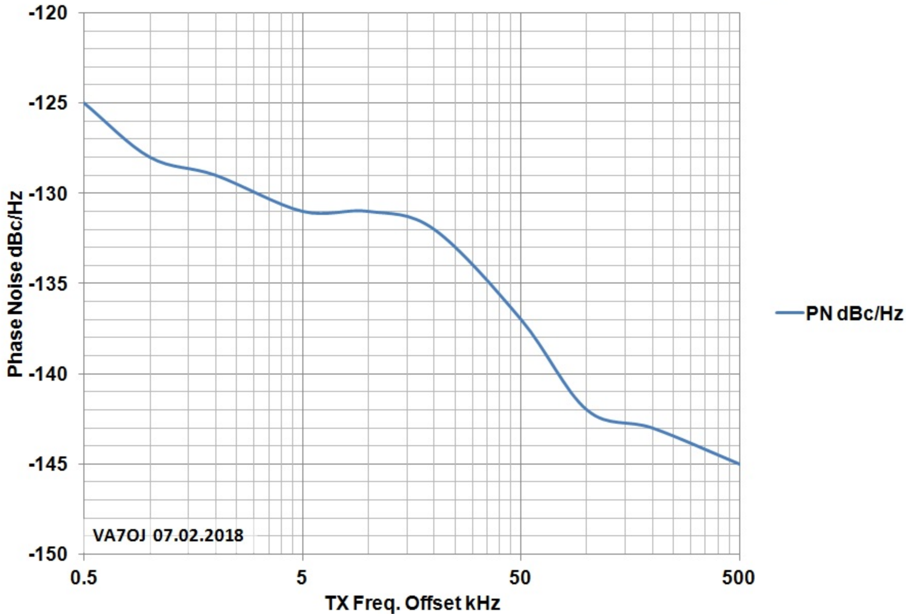
IC-7610 XVTR TX Phase Noise dBc/Hz at 28.1 MHz. Po = 100%
